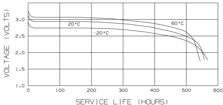
Typical Temperature Characteristics K123LA
