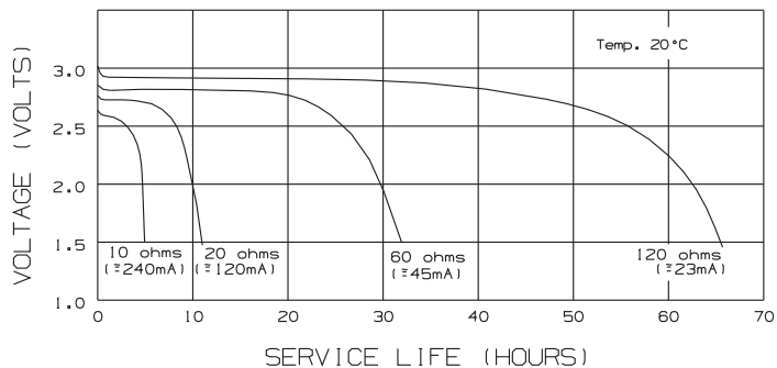
Typical Discharge Characteristics K123LA
